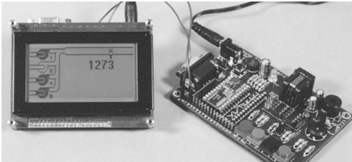
Figure 5. Photo of G12864 graphics-display demo driven by BS2 on Stamp Activity Board.
